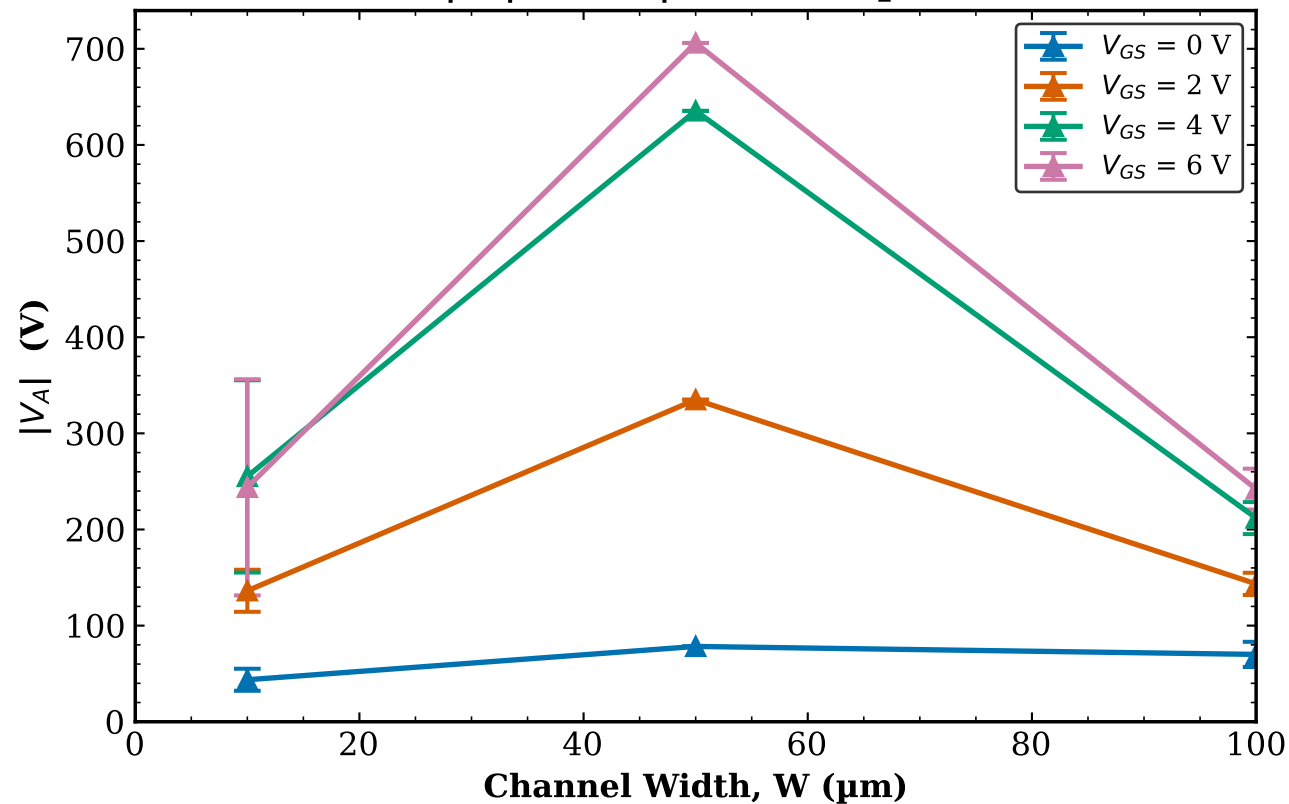
TFT1 Combined (Tr. 1 & 2) |V_A| vs W | L = 160\text{ }\mu\text{m}
